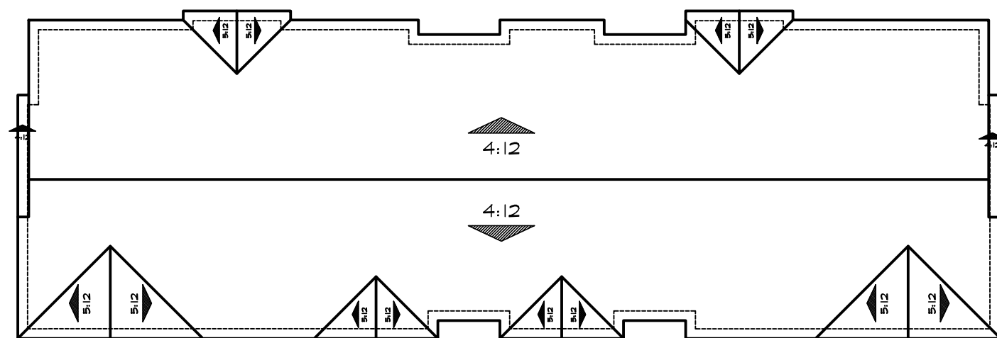
Roof Plan
