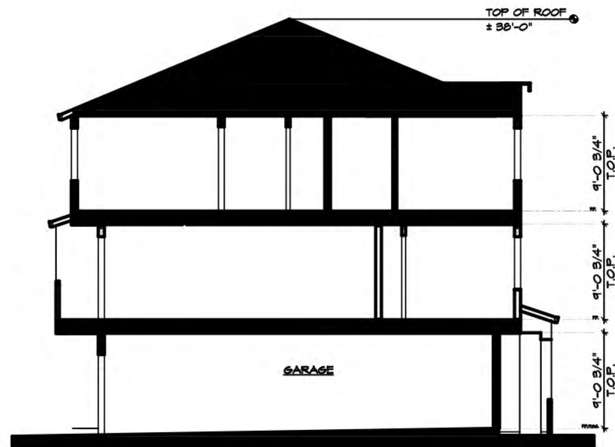
Typical Cross Section
