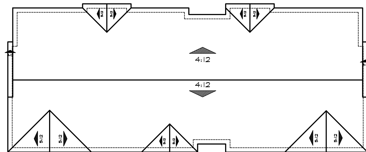
Roof Plan
