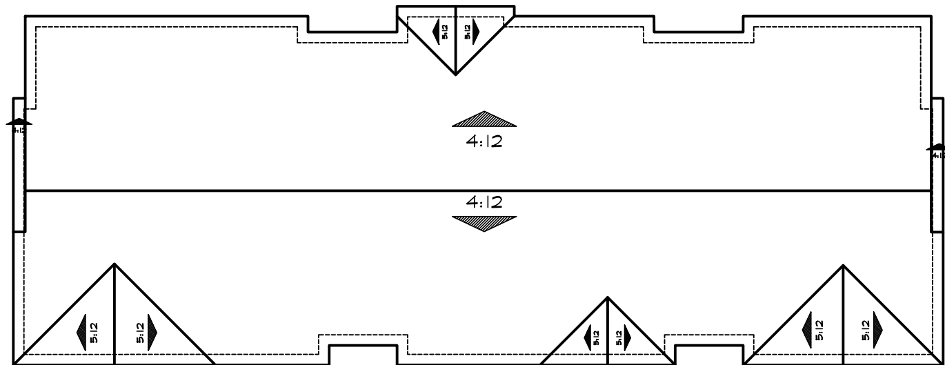
Roof Plan
