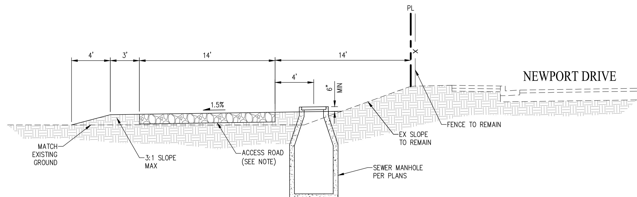
SECTION A NOT TO SCALE
