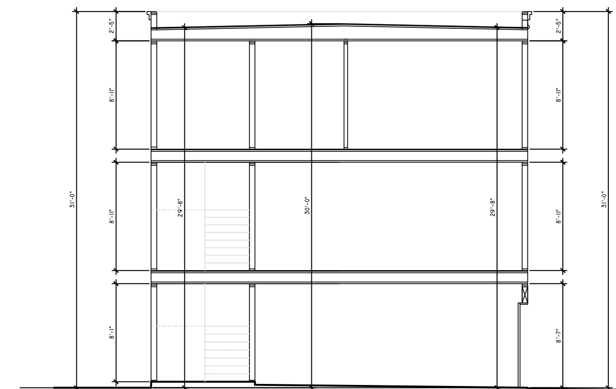
SECTION THRU TYP. UNIT
